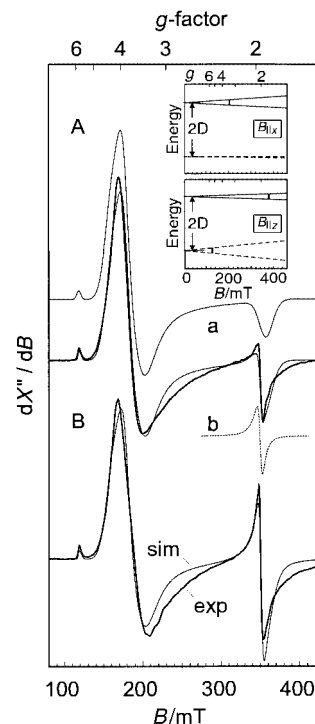
Fig. 1 (A) X-Band EPR spectra of [(\text{H}_2\text{O})_5\text{Cr}^{\text{III}}-\text{CHCl}_2]^{2+} . Experimental conditions: microwave frequency 9.6529 GHz, microwave power 100 \mu\text{W} , modulation amplitude 1.1 mT, temperature 7 K. The simulation (thin line) is a superposition of subspectra (a) and (b) with spin-Hamiltonian parameters for a: D = -1.6 \text{ cm}^{-1} , E/D = 0.057 , \sigma(E/D) = 0.033 , g = \{1.967, 1.967, 1.95\} , Gaussian lines with frequency-dependent linewidth W_f = 40 \text{ mT} and an additional angular-dependent contribution in the y direction W_y = 18 \text{ mT} ; b is a single-line approximation of the spectral contribution from ‘free’ chromium hexaaqua complexes with effective g value 1.98 (2% integral intensity). Inset: energies of the magnetic sublevels of the S = 3/2 manifold as a function of the field applied in the molecular x and z directions for D = -1.6 \text{ cm}^{-1} , E/D = 0.06 . (B) X-Band EPR spectrum of [(\text{H}_2\text{O})_5\text{Cr}^{\text{III}}-\text{CHBr}_2]^{2+} . Experimental conditions: microwave frequency 9.6545 GHz, microwave power 100 \mu\text{W} , modulation amplitude 1.1 mT, temperature 5 K. The simulation is a superposition of the subspectra a and b as described for (A), but with W_f = 50 \text{ mT} , W_y = 0 for a and 12% intensity for b.
